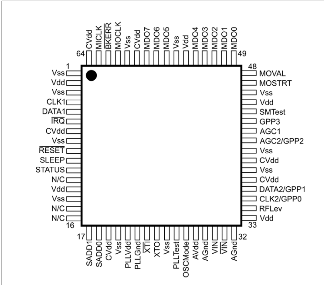
Figure 2 - Pin Outline
