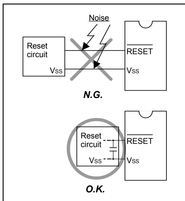
Fig 70. Wiring for the \overline{\text{RESET}} pin
