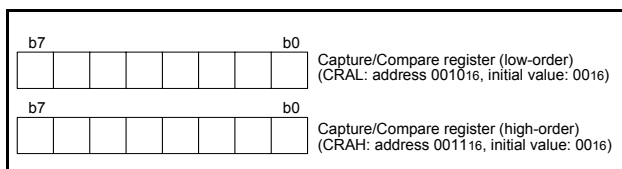
Fig 26. Structure of capture/compare register
