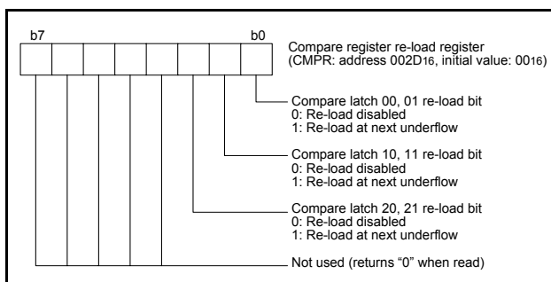
Fig 28. Structure of compare register re-load register
