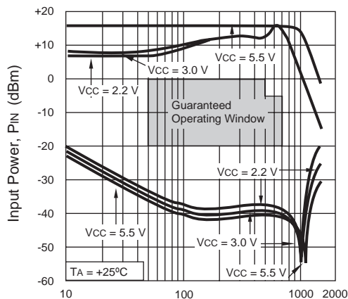
INPUT POWER vs. INPUT FREQUENCY and VOLTAGE
