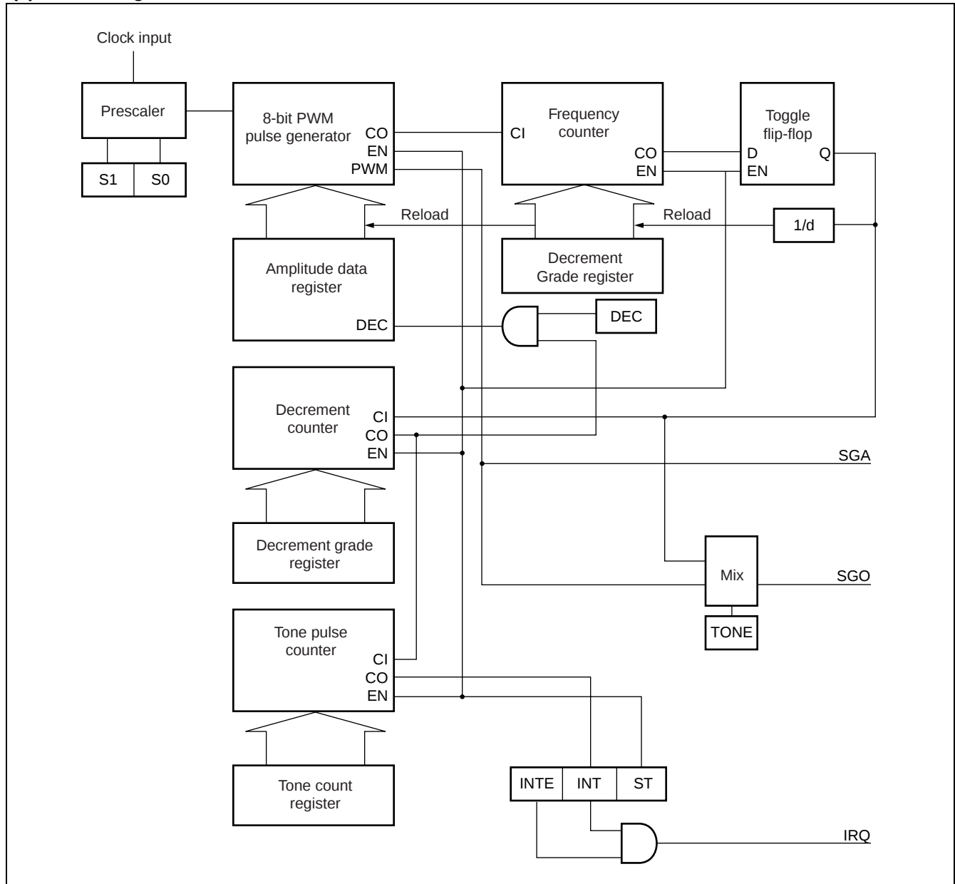
(2) Block Diagram
