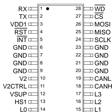
Figure 3. 33989 Pin Connections
