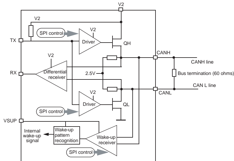
Figure 34. 33989 CAN Interface
