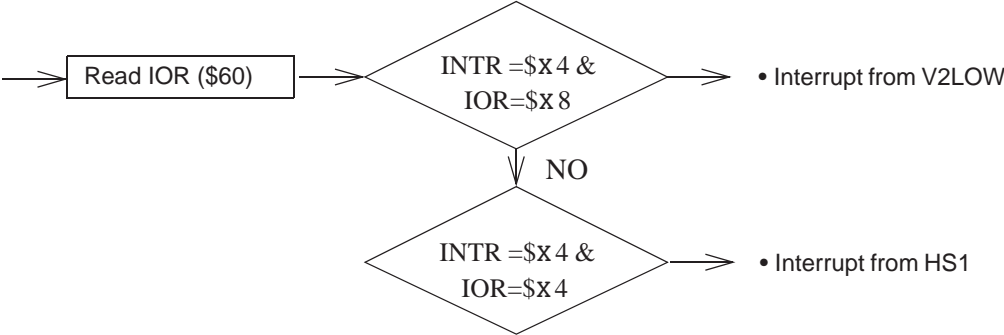
Figure 61. Distinguish Between V2LOW and HS1 Overtemperature
