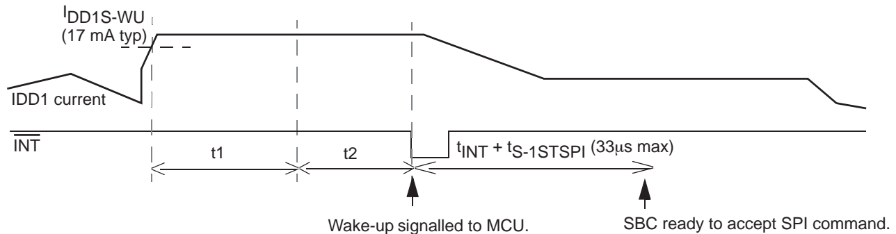
Figure 32. Overcurrent Wake-Up
