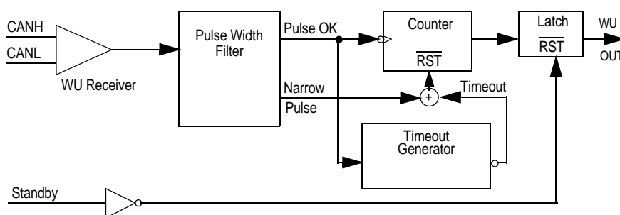
Figure 4. Wake-Up Block Diagram
