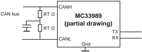
Split termination concept
