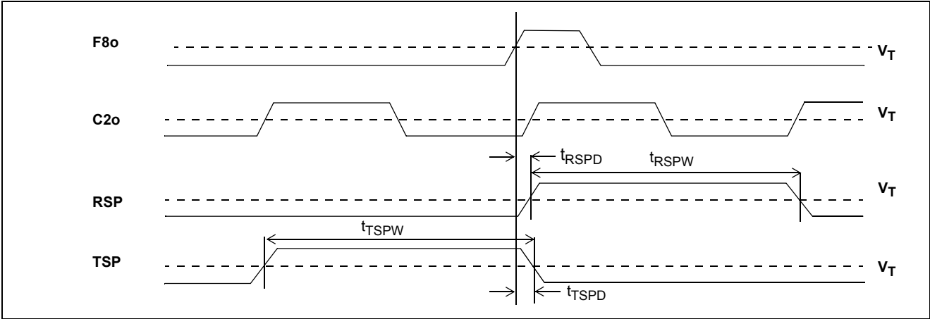
Figure 16 - Output Timing 2
