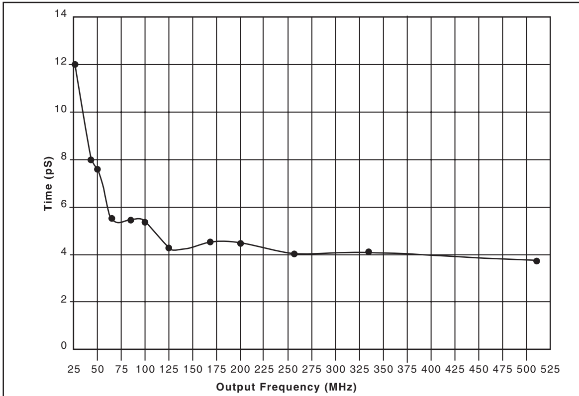
FIGURE 4A. RMS JITTER vs. f_{OUT} (using a 16MHz XTAL)
