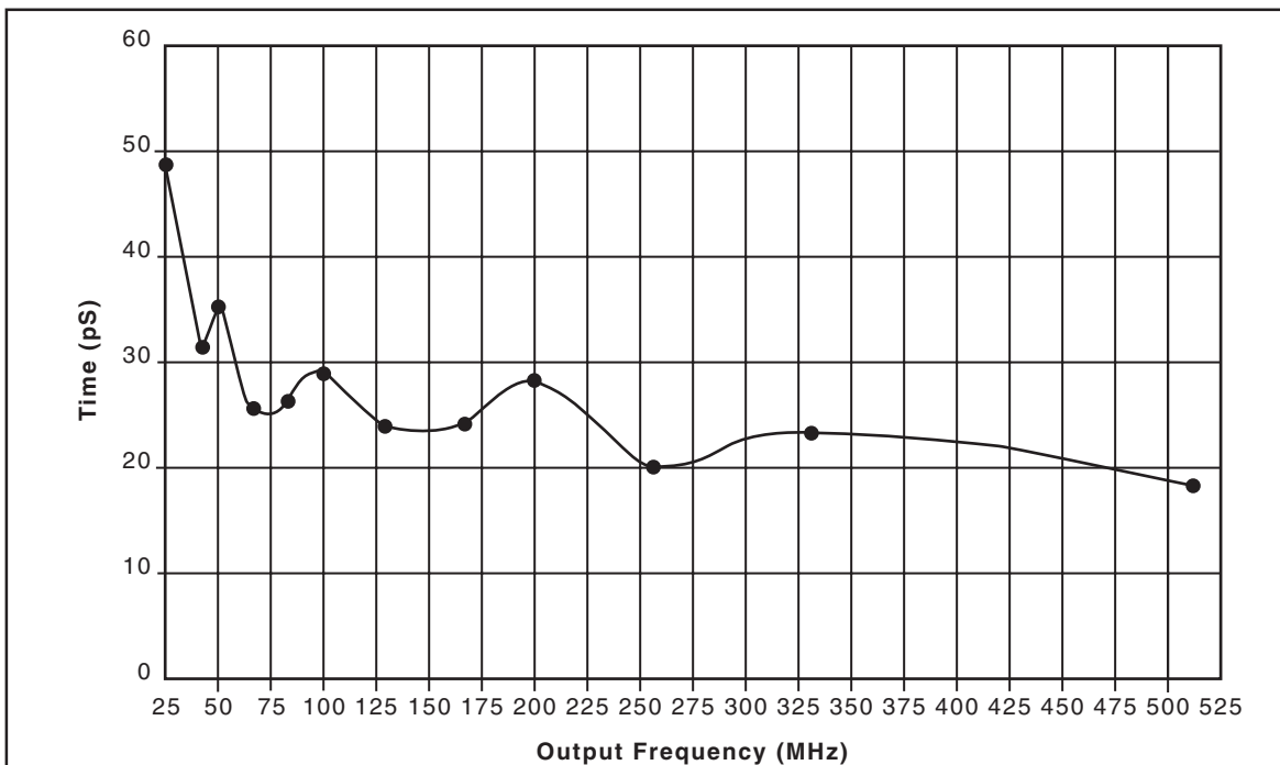
FIGURE 4B. CYCLE-TO-CYCLE JITTER vs. f_{OUT} (using a 16MHz XTAL)
