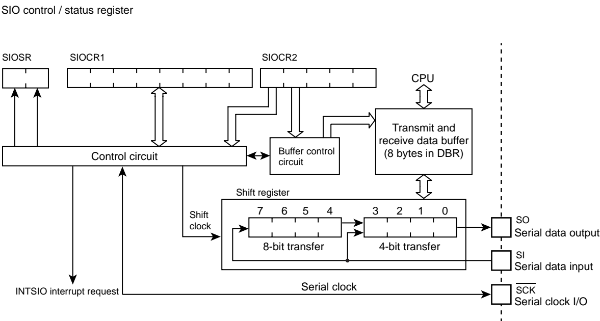
Figure 12-1 Serial Interface
