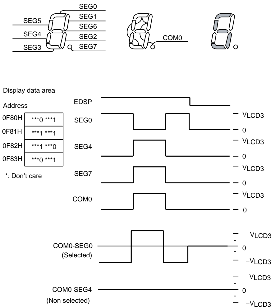
Figure 15-11 Static Drive
