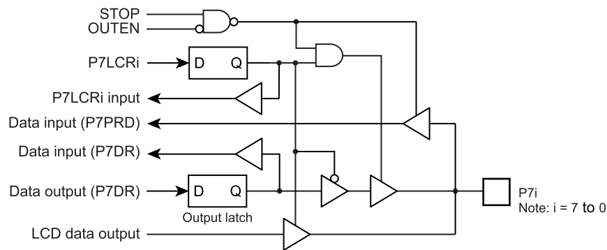
Figure 5-7 Port P7
