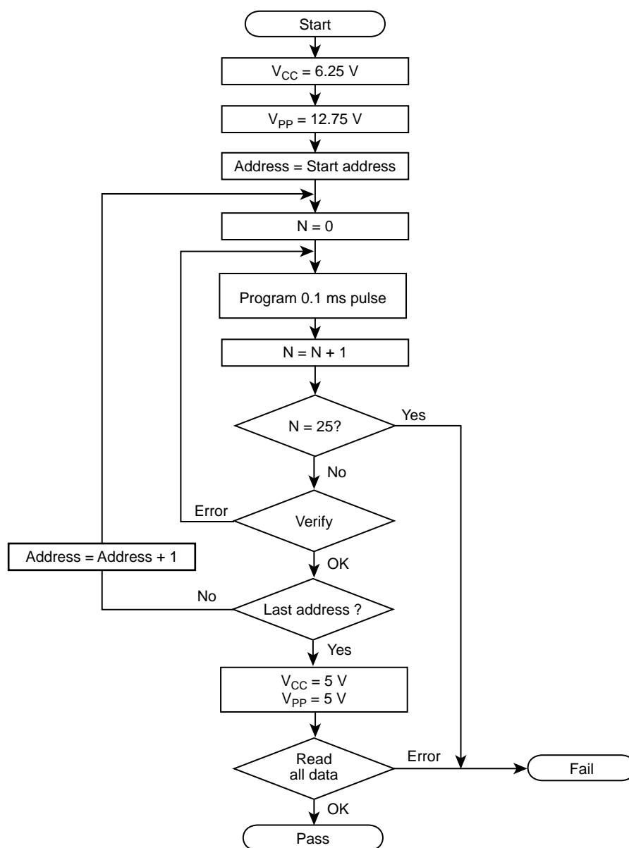
Figure 16-3 Programming Flowchart
