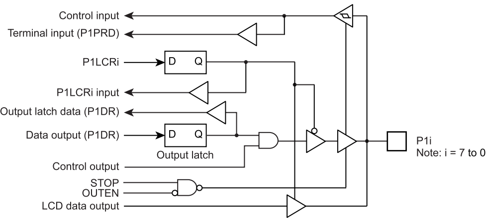
Figure 5-2 Port P1
