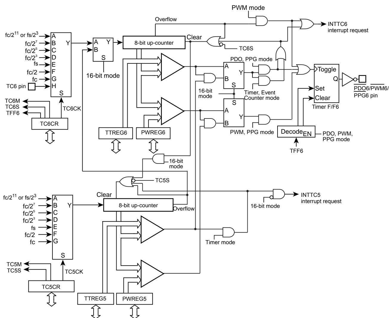
Figure 10-1 8-Bit TimerCounter 5, 6
