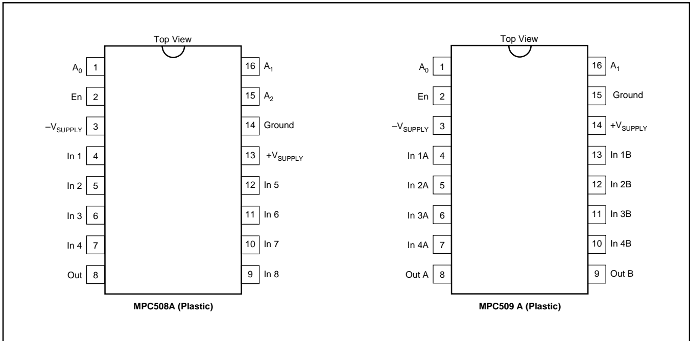
MPC508A
