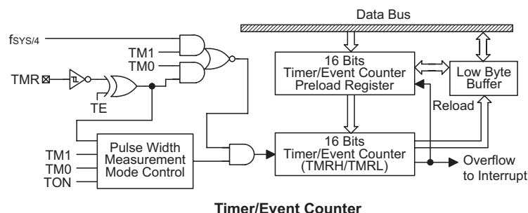
Timer/Event Counter
