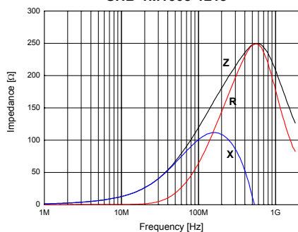
SHB-1M1608-121J
