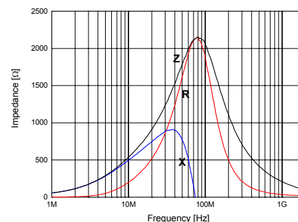
SHB-1T1608-202J
