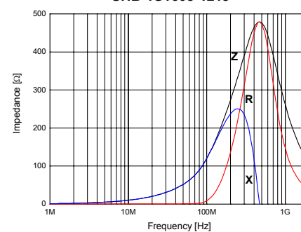
SHB-1S1608-121J
