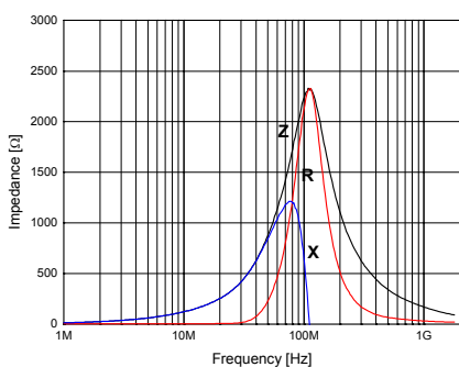
SHB-1B1608-222J
