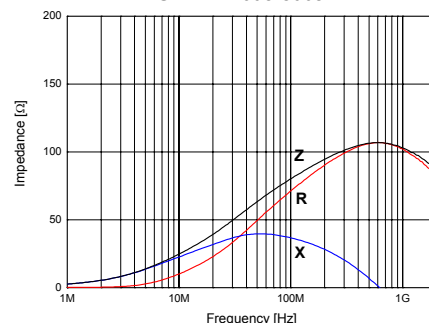
SHB-1T1608-800J
