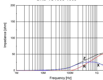
SHB-1S1608-100J
