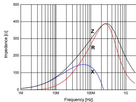
SHB-1T1608-301J
