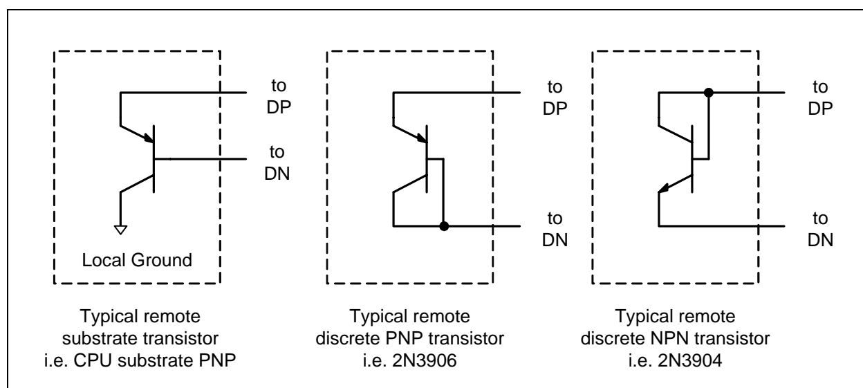
Figure 4.4 Diode Connections
