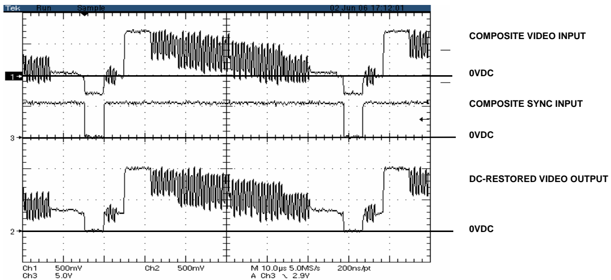
FIGURE 15. DC-RESTORE USING COMPOSITE SYNC AND V_{REF} = 0VDC
