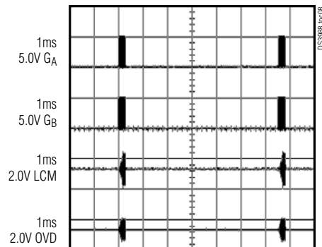
BURST DIMMING AT 150Hz AND 10%
