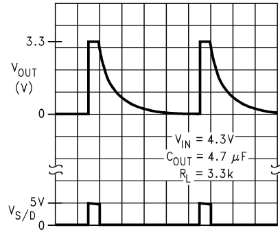
Turn-On Waveform
