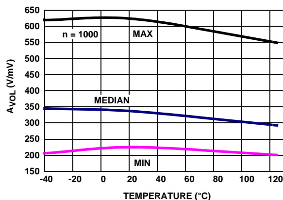
FIGURE 24. A_{VOL} vs TEMPERATURE V_+ , V_- = \pm 2.5V , R_L = 100k\Omega
