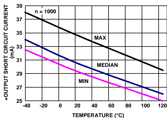
FIGURE 32. +OUTPUT SHORT CIRCUIT CURRENT vs TEMPERATURE V_{IN} = +2.5V , R_L = 10\Omega , V_+ = 5V , V_- = 0V
