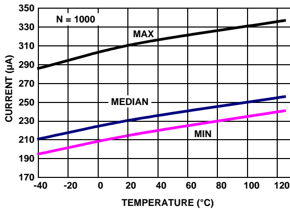
FIGURE 15. ISL28488 SUPPLY CURRENT vs TEMPERATURE V_+ , V_- = \pm 2.5V ENABLED, R_L = \text{INF}
