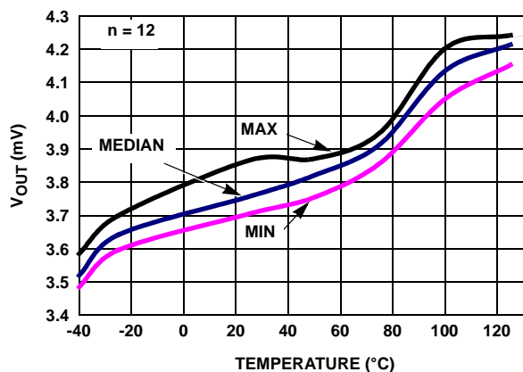
FIGURE 31. V_{OUT\ LOW} vs TEMPERATURE, V_+ = 5V , V_- = 0V , R_L = \text{Open}
