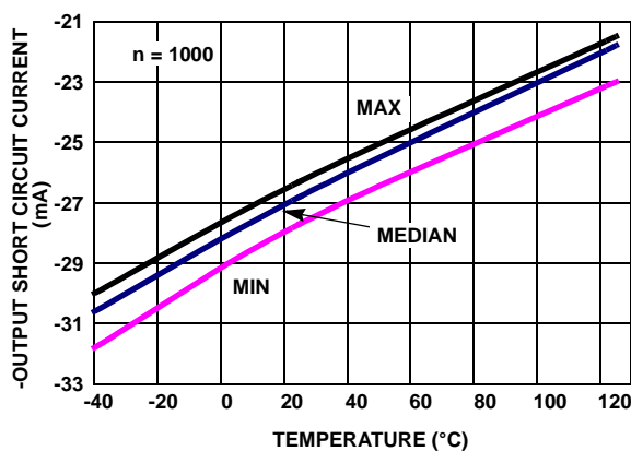
FIGURE 33. -OUTPUT SHORT CIRCUIT CURRENT vs TEMPERATURE V_{IN} = -2.5V , R_L = 10\Omega , V_+ = 5V , V_- = 0V
