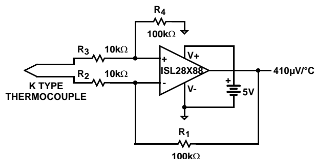
FIGURE 36. THERMOCOUPLE AMPLIFIER
