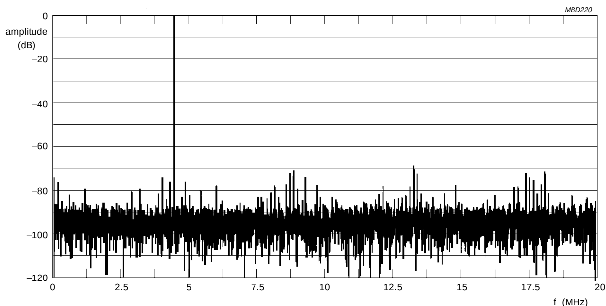
Fig.9 Fast Fourier Transformer ( f_{\text{clk}} = 40 \text{ MHz} ; f_i = 4.43 \text{ MHz} ); for differential input mode.
