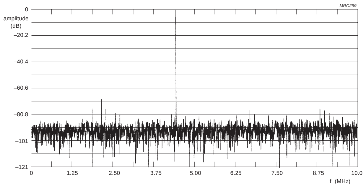
Fig.8 Fast Fourier Transformer ( f_{\text{clk}} = 20 \text{ MHz} ; f_i = 4.43 \text{ MHz} ); for differential input mode.
