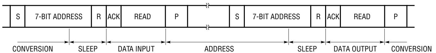
Figure 7. Consecutive Reading with the Same Input/Configuration
