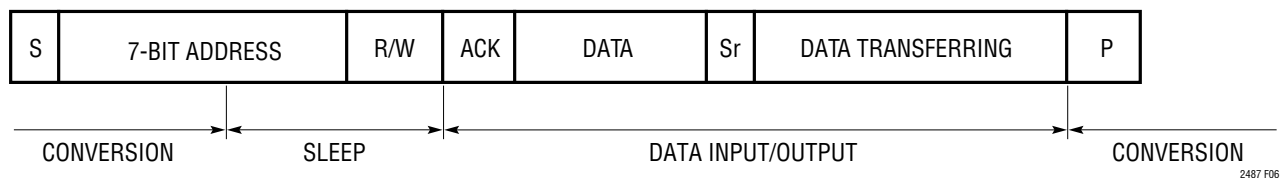
Figure 6. Conversion Sequence
