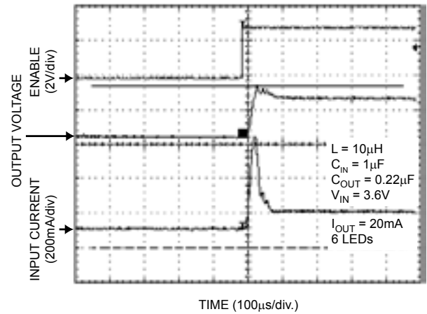
6-Series LED Circuit without External Soft-Start
