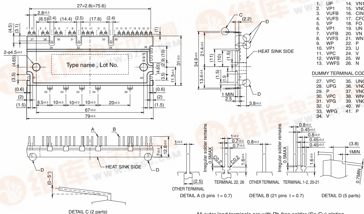
Fig. 1 PACKAGE OUTLINES (Short-pin type : PS21869-P) Refer Fig. 6 for long-pin type : PS21869-AP.
