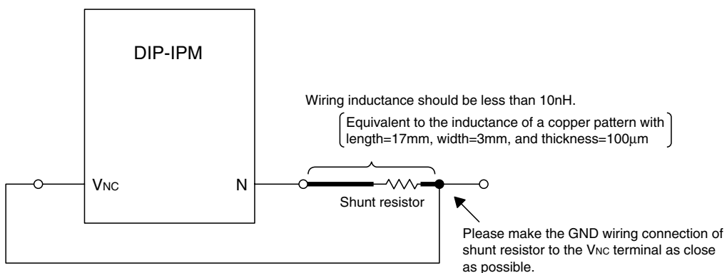
Fig. 9 WIRING CONNECTION OF SHUNT RESISTOR
