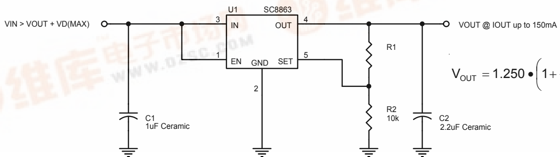
Externally Preset Output Voltage (4)
