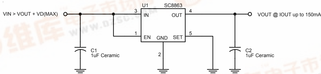
Internally Preset Output Voltage
