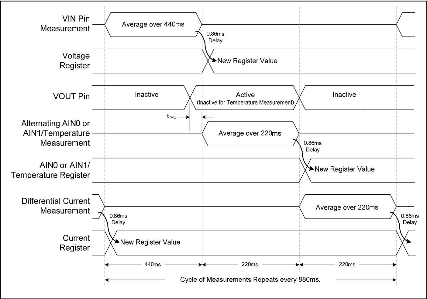
Figure 4. Measurement Sequence
