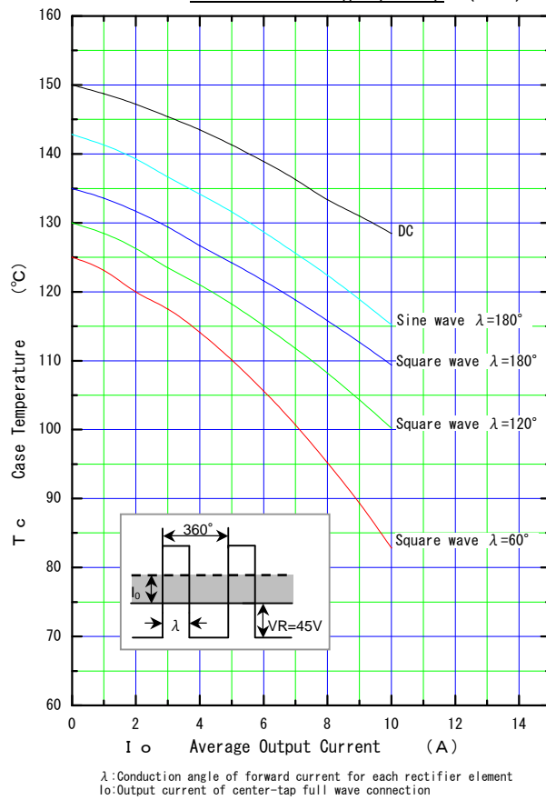
Current Derating ( I_o - T_c ) (max.)
