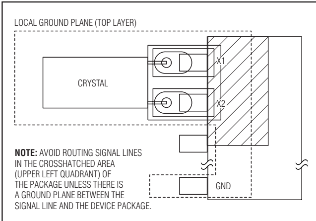
Figure 3. Layout Example
