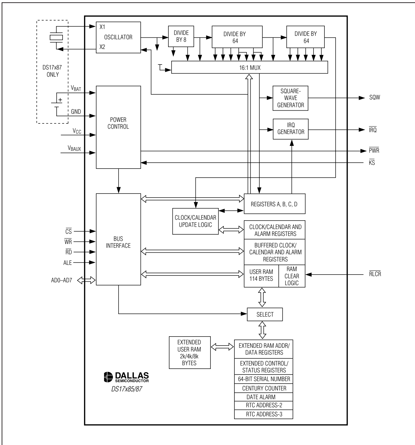
Figure 1. Functional Diagram
