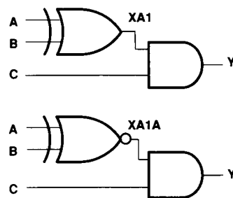
Figure 14. XOR-AND/ XNOR-AND Gates
