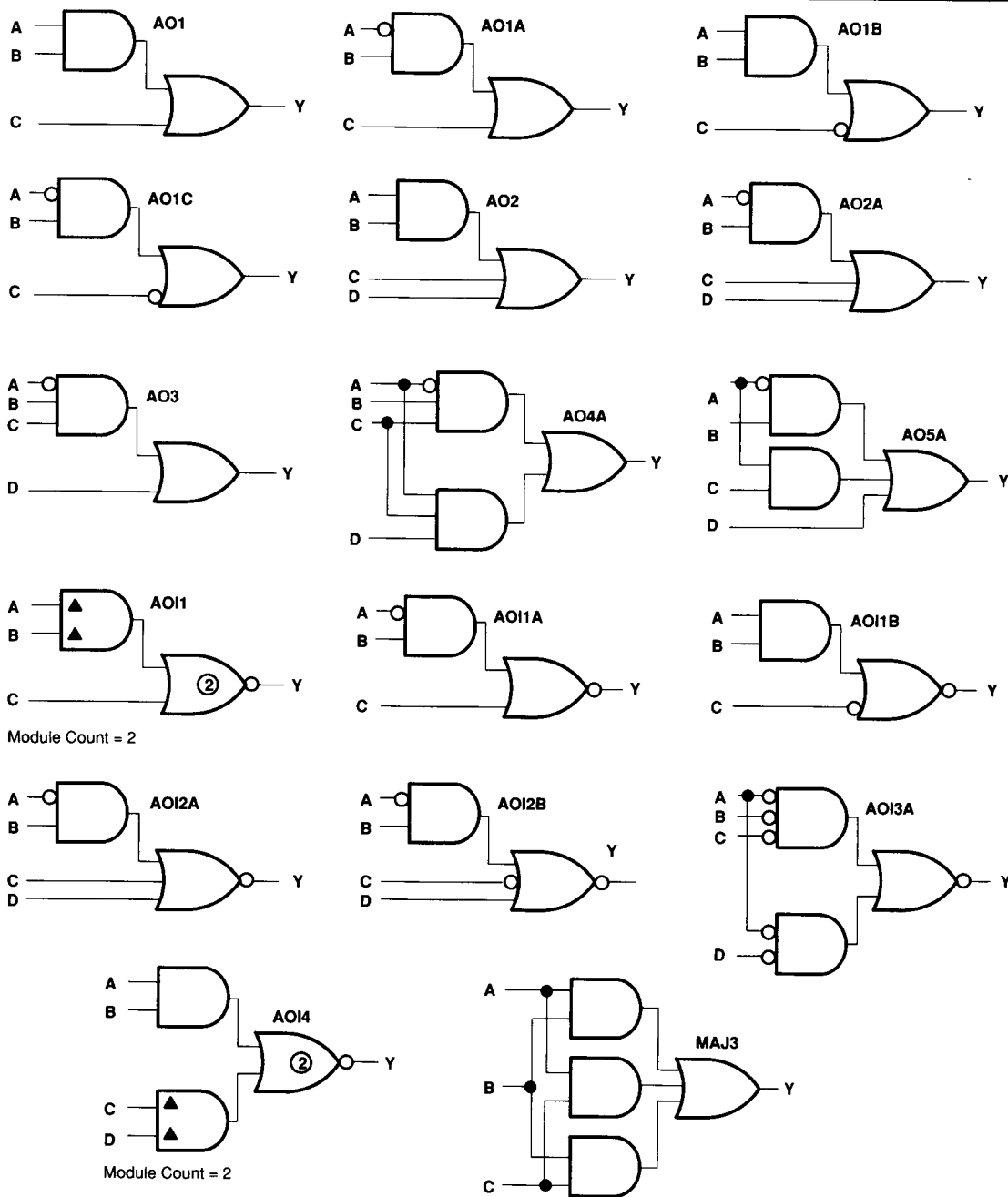
Figure 16. AND-OR/AND-NOR Gates
