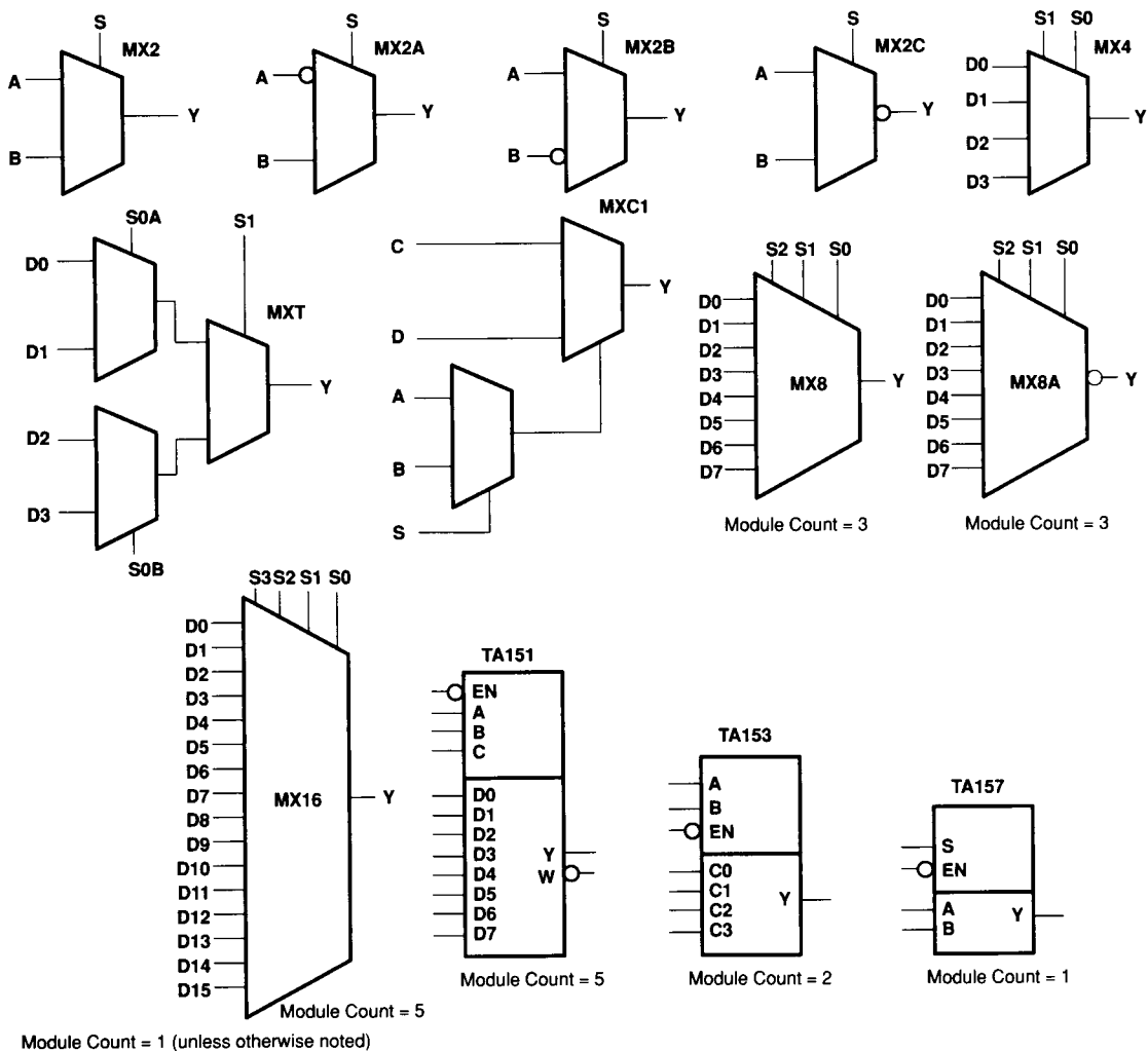
Figure 20. Multiplexers
