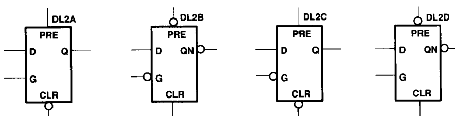
Figure 22. D-Type Latches
