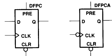
Figure 23. D-Type Flip-Flops
