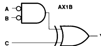
Figure 14. XOR-AND/ XNOR-AND Gates
