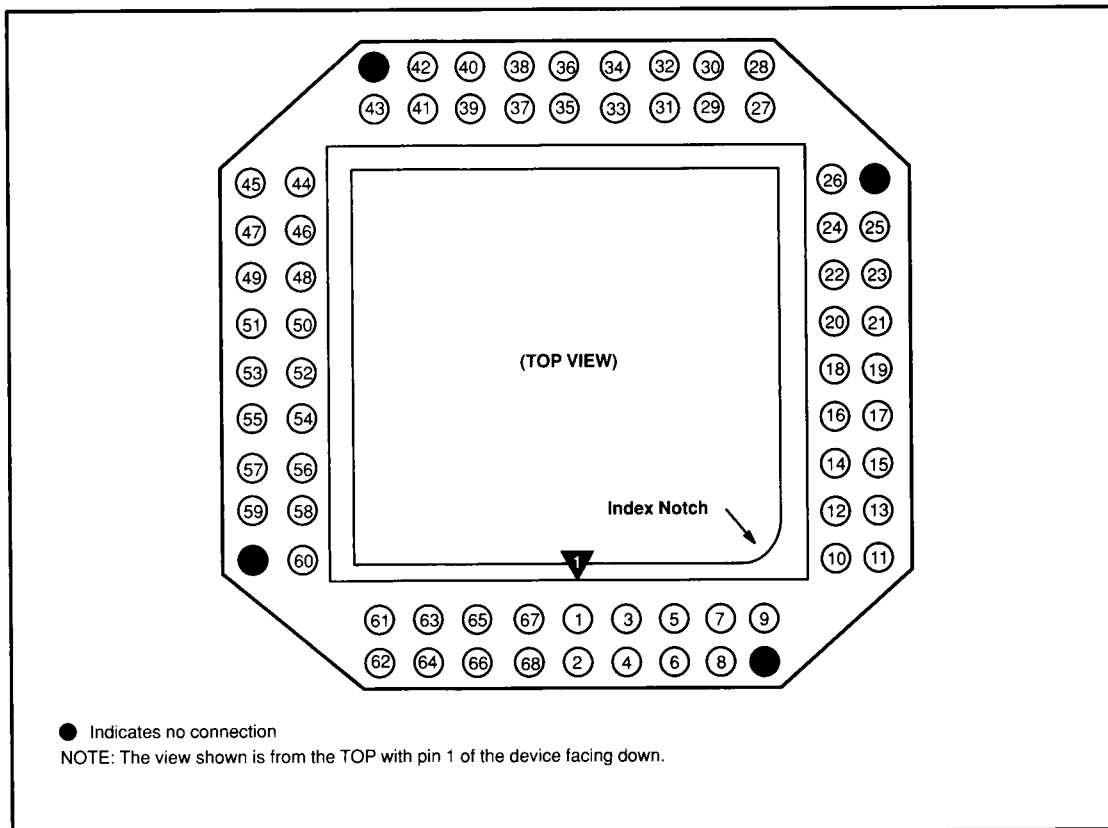
Figure 44. 68-Pin PLCC Actionprobe
