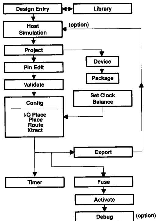
Figure 1. Design Flow
