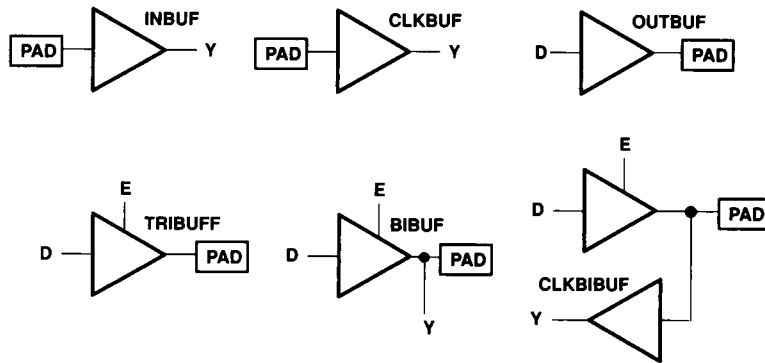
Figure 19. I/O Buffers
