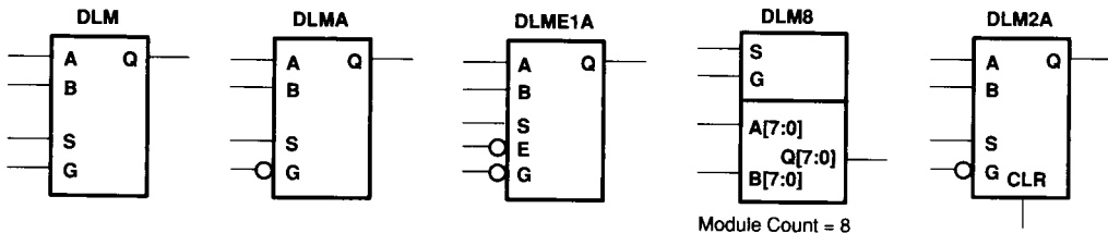
Figure 22. D-Types Latches (Continued)
