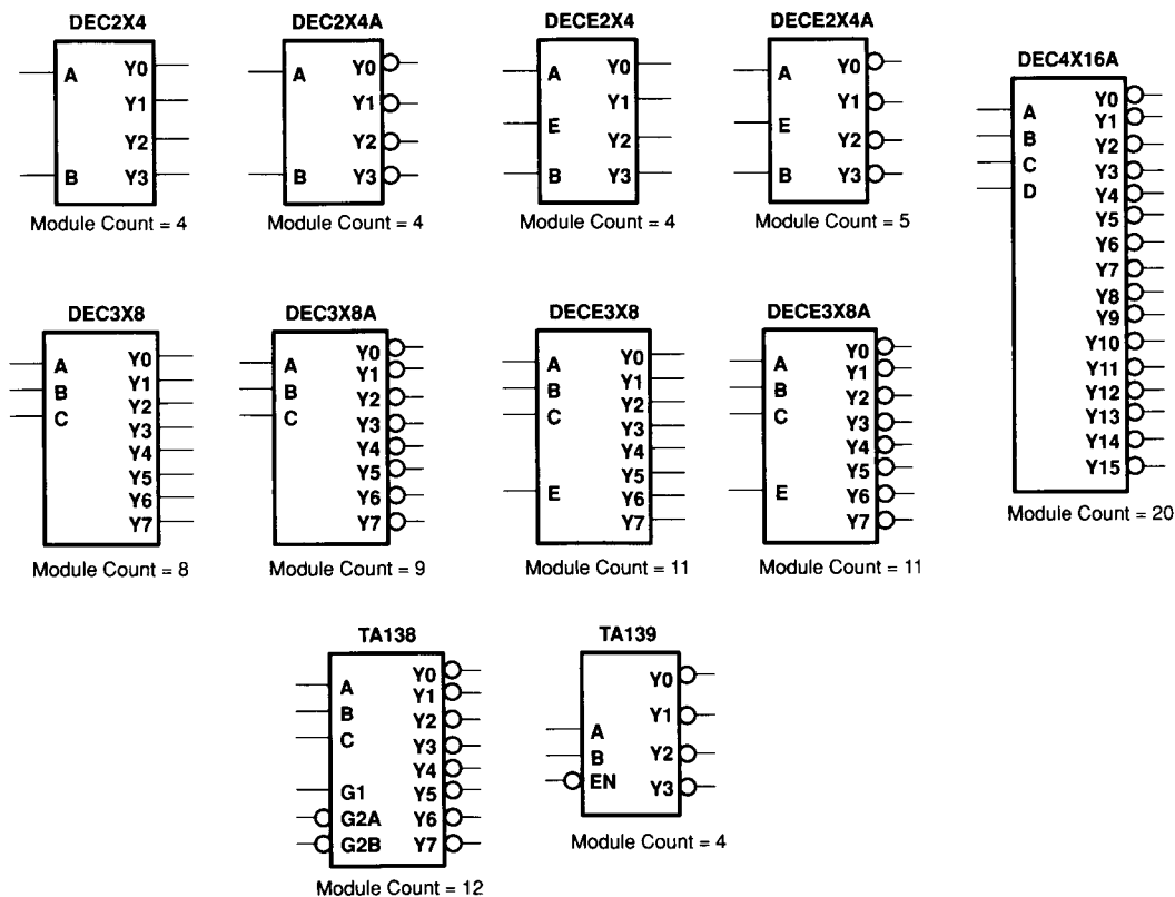
Figure 31. Decoders
