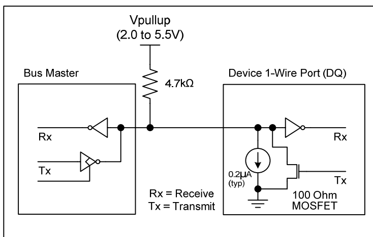
Figure 8. 1-Wire Bus Interface Circuitry
