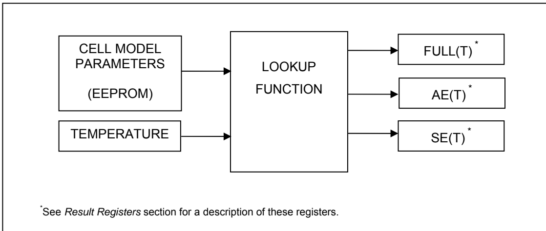
Figure 4. Lookup Function Diagram
