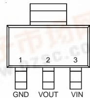
SOT-223 (F-Type)
