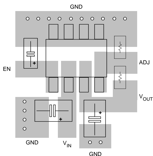
SOP-8 Board Layout
