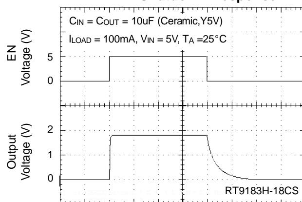
EN Pin Shutdown Response
