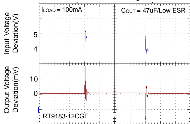
Line Transient Regulation
