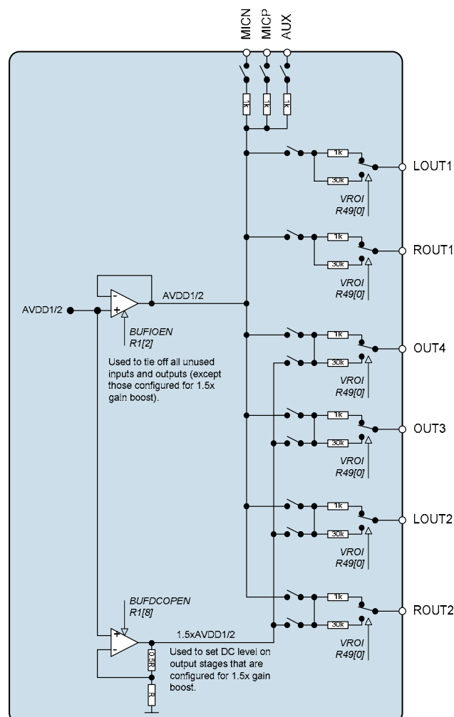
Figure 41 Unused Input/Output Pin Tie-off Buffers
