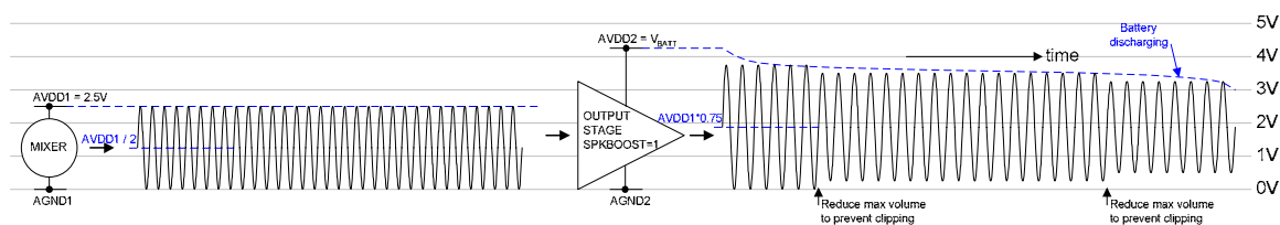
Figure 37 Output Boost Mode with Direct Battery Connection
