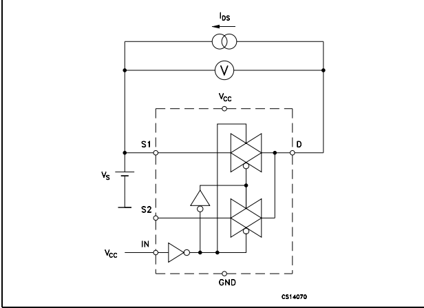
Figure 5. OFF Leakage
