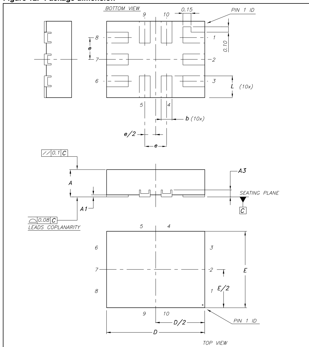
Figure 12. Package dimension
