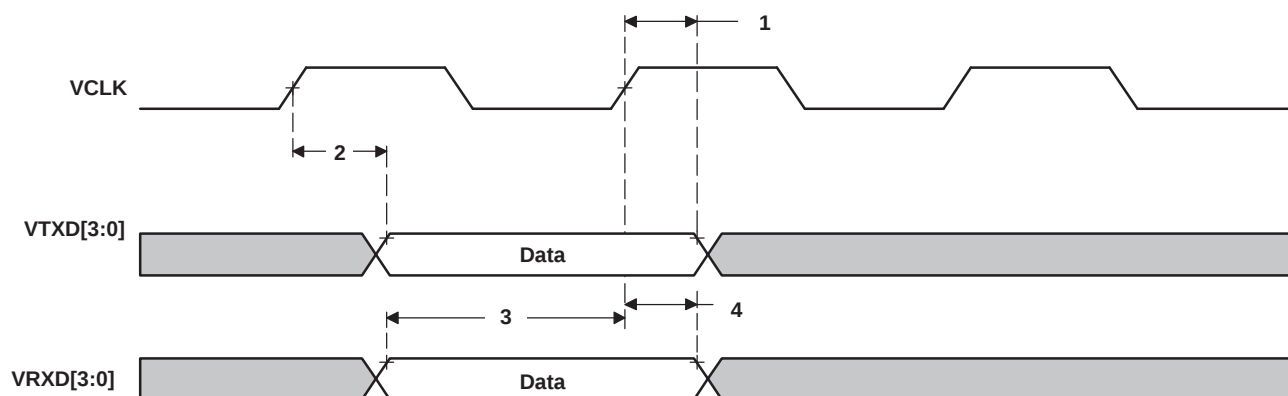
Figure 6-45. VLYNQ Transmit/Receive Timing
