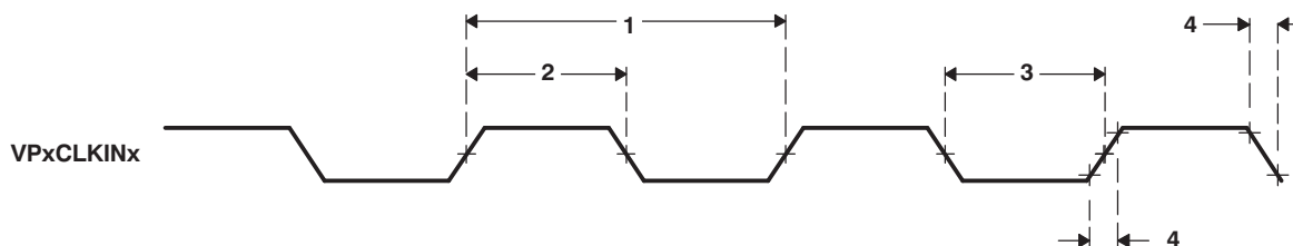
Figure 6-23. Video Port Display VPxCLKINx Timing
