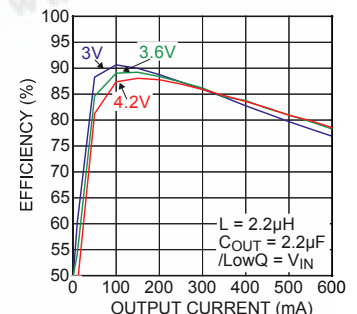
DC/DC 1.8V OUT Efficiency
