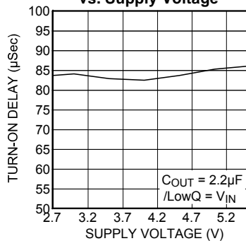
DC/DC Turn-On Delay vs. Supply Voltage
