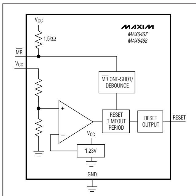
Figure 2. Functional Diagram
