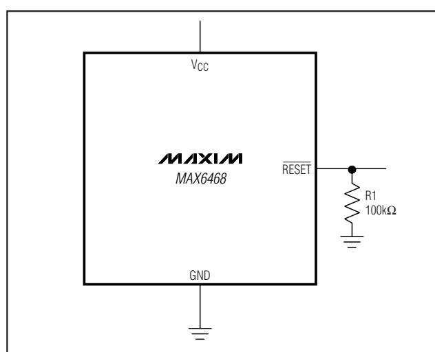
Figure 3. RESET Valid to V CC = 0V
