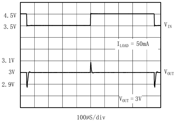
Line-Transient Response
