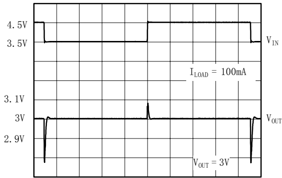
Line-Transient Response
