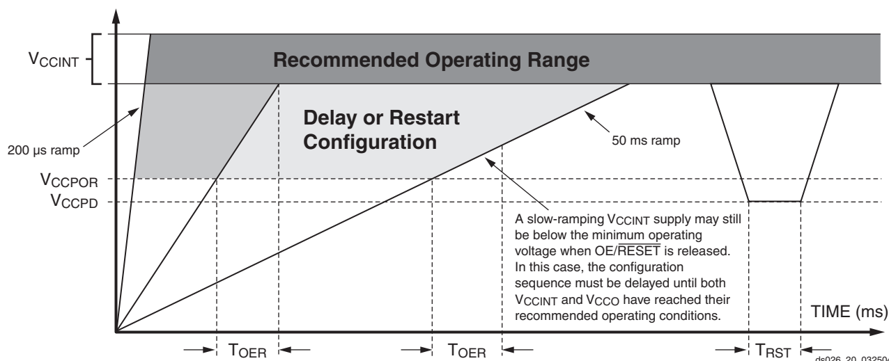
Figure 9: V_{CCINT} Power-Up Requirements
