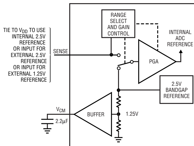
Figure 6. Reference Circuit
