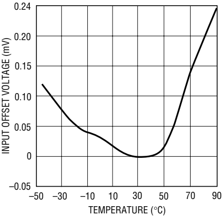
Input Offset Voltage Drift vs Temperature, Drift from 25°C
