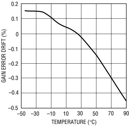
Gain Error Drift vs Temperature, Internal Reference, Drift from 25°C
