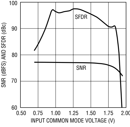
SNR and SFDR vs Input Common Mode Voltage
