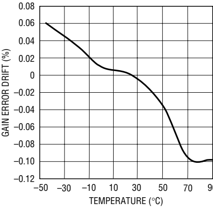
Gain Error Drift vs Temperature, External Reference, Drift from 25°C
