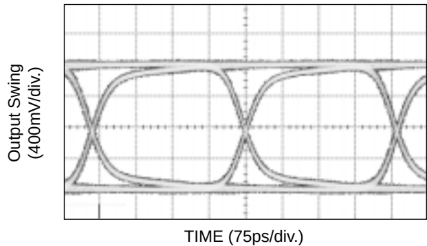
3.2Gbps Output (Q – I/Q)
