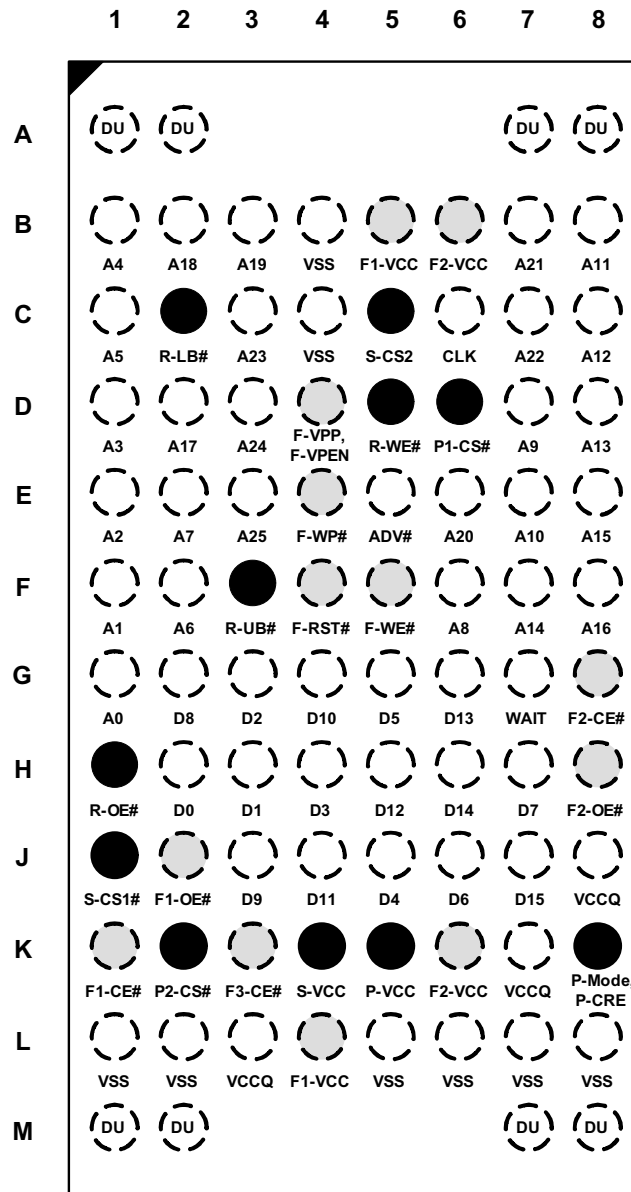
Top View - Ball Side Down
