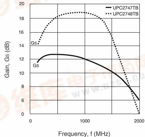
GAIN vs. FREQUENCY V_{CC} = 3.0 V
