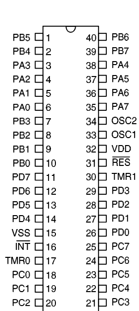
HT48C50/HT48C70 – 40 DIP-A
