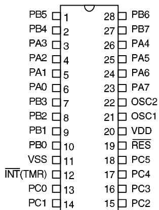
HT48C30 – 28 SKDIP-B
