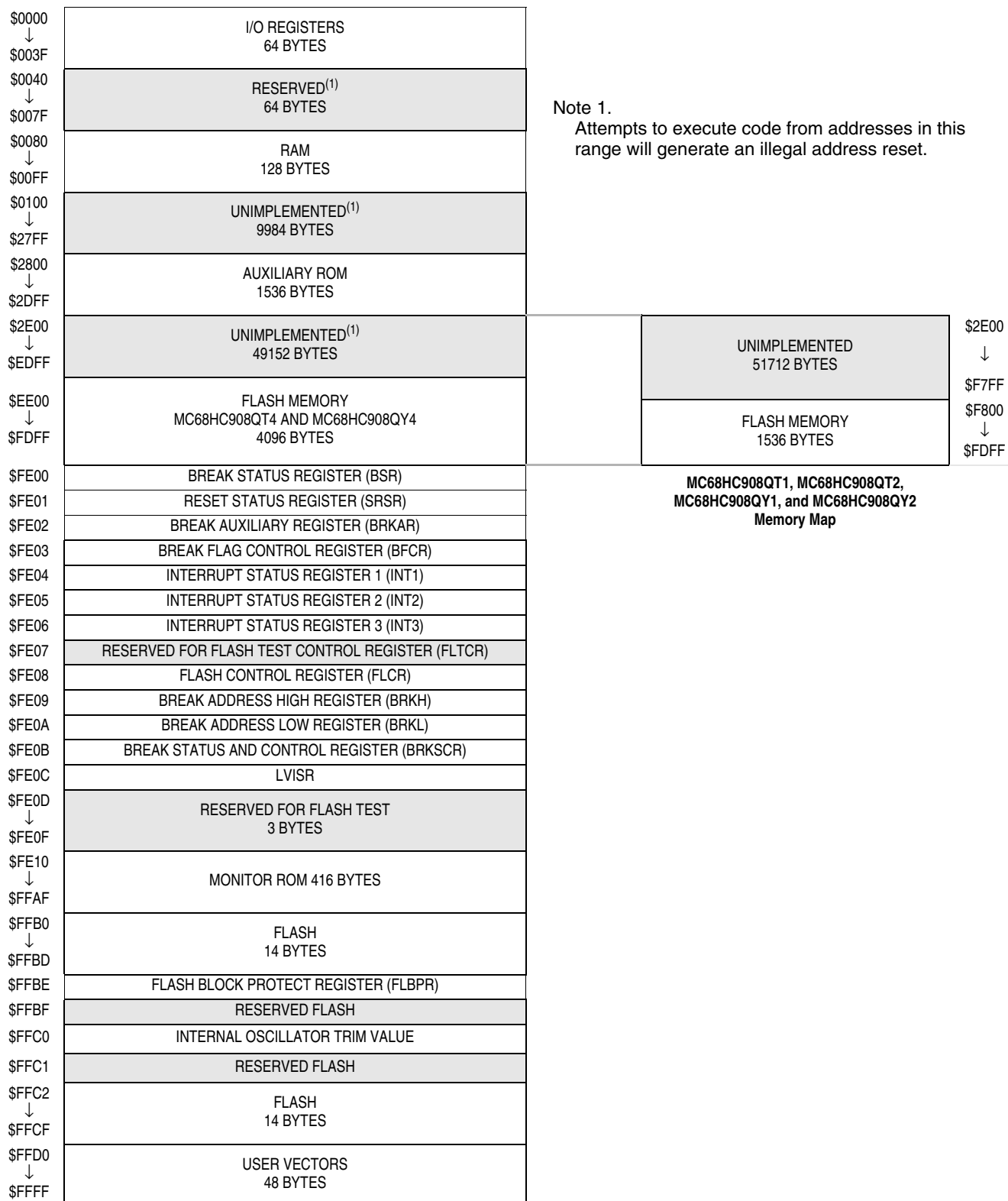
Figure 2-1. Memory Map
