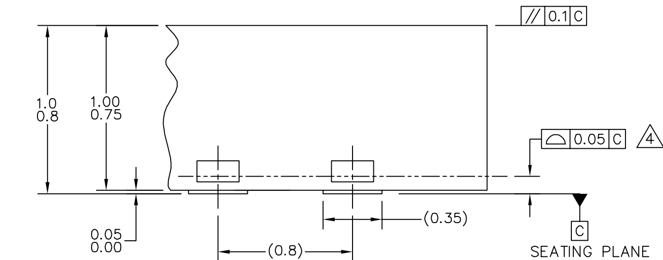
DETAIL G
