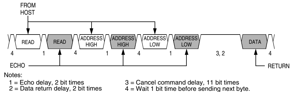
Figure 15-15. Read Transaction
