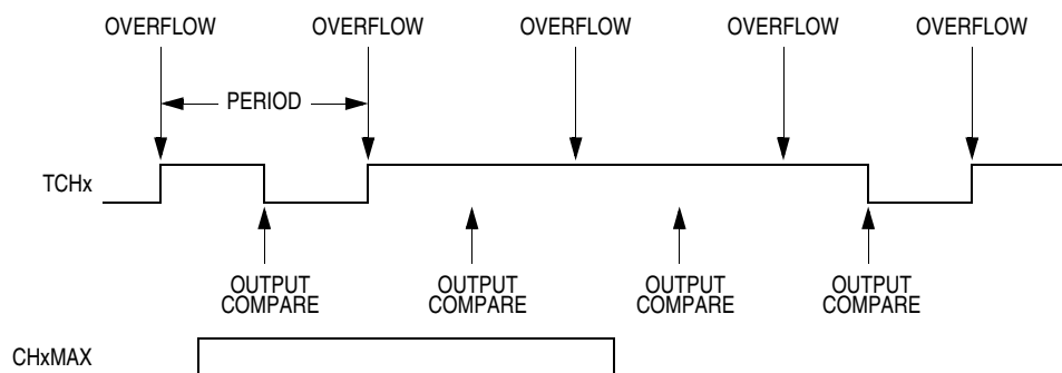
Figure 14-8. CHxMAX Latency
