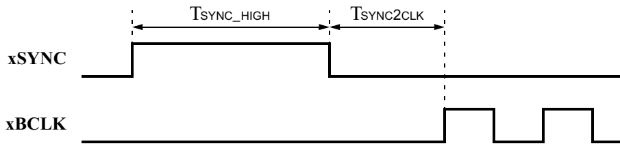
Figure 5-2. Warm Reset Timing
