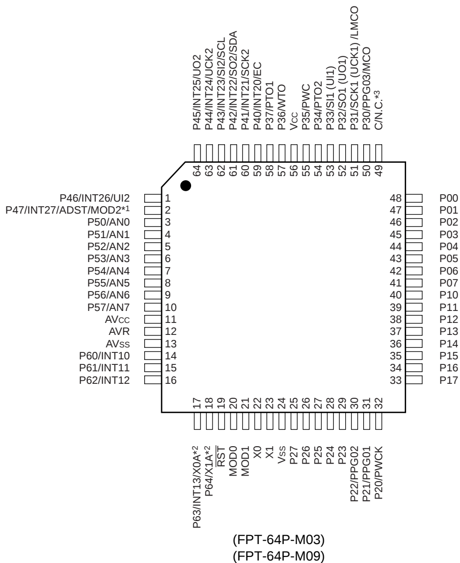
(TOP VIEW)
