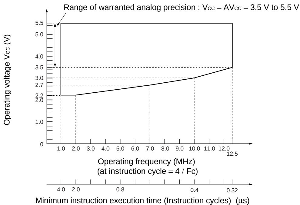
Operating voltage vs. operating frequency (MB89535A/537A/538A/537AC/538AC)
