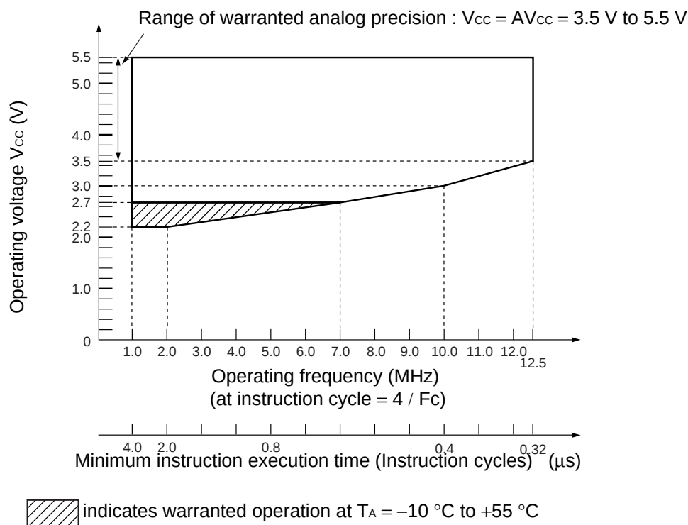
Operating voltage vs. operating frequency (MB89P538/MB89PV530)
