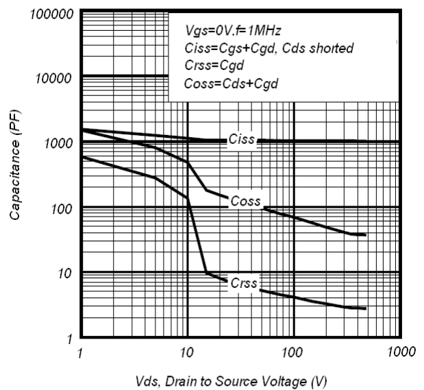
Fig 8. Capacitance Characteristics
