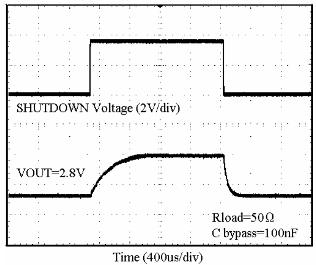
SHUTDOWN RESPONSE WAVEFORM (CBP=100nF)
