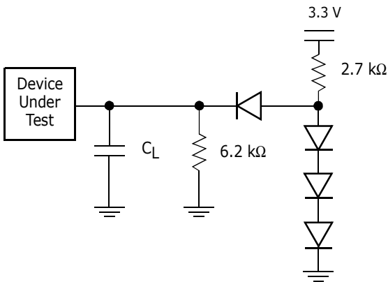
Figure II. Test Setup
