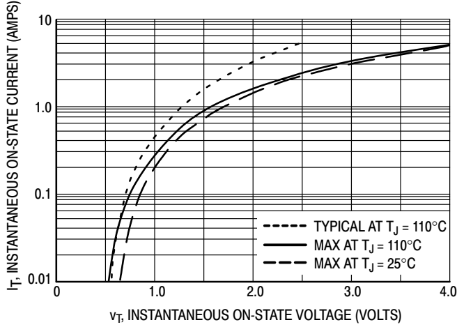
Figure 2. On-State Characteristics
