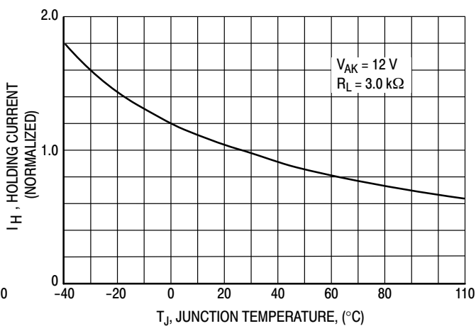
Figure 11. Typical Normalized Holding Current versus Junction Temperature
