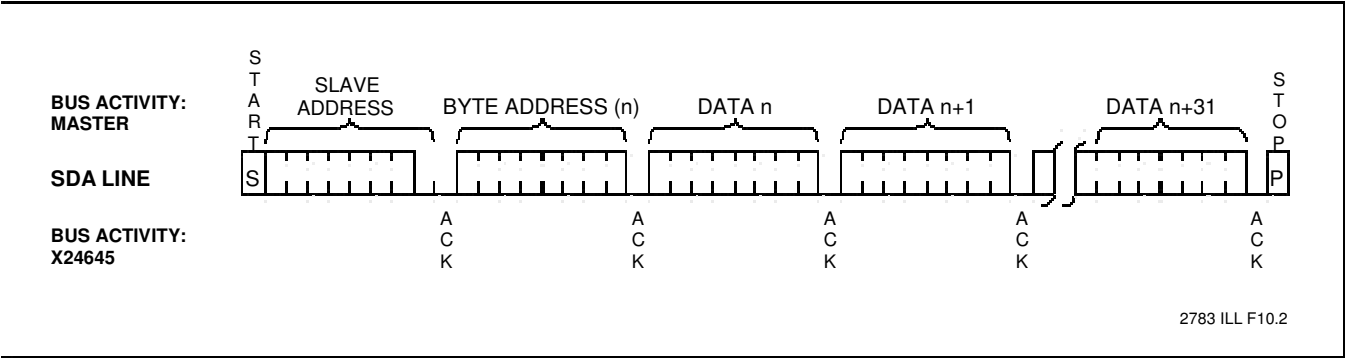
Figure 6. Page Write
