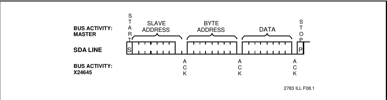
Figure 5. Byte Write
