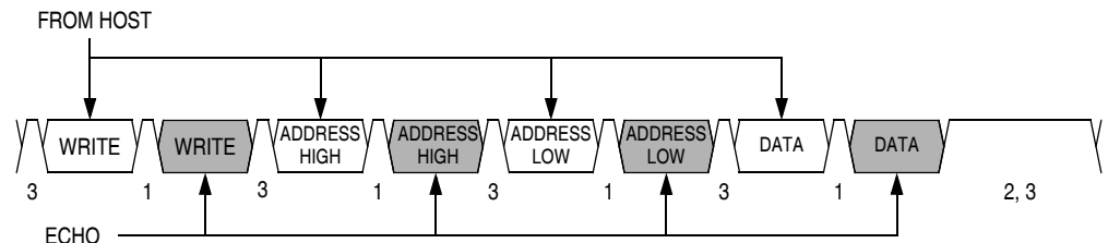
Figure 10-5. Read Transaction
