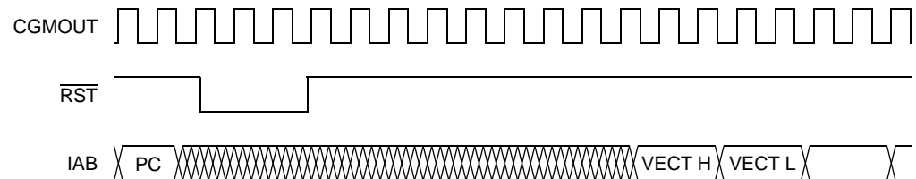
Figure 9-4. External Reset Timing
