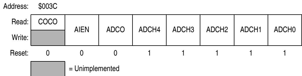
Figure 15-4. ADC Status and Control Register (ADSCR)
