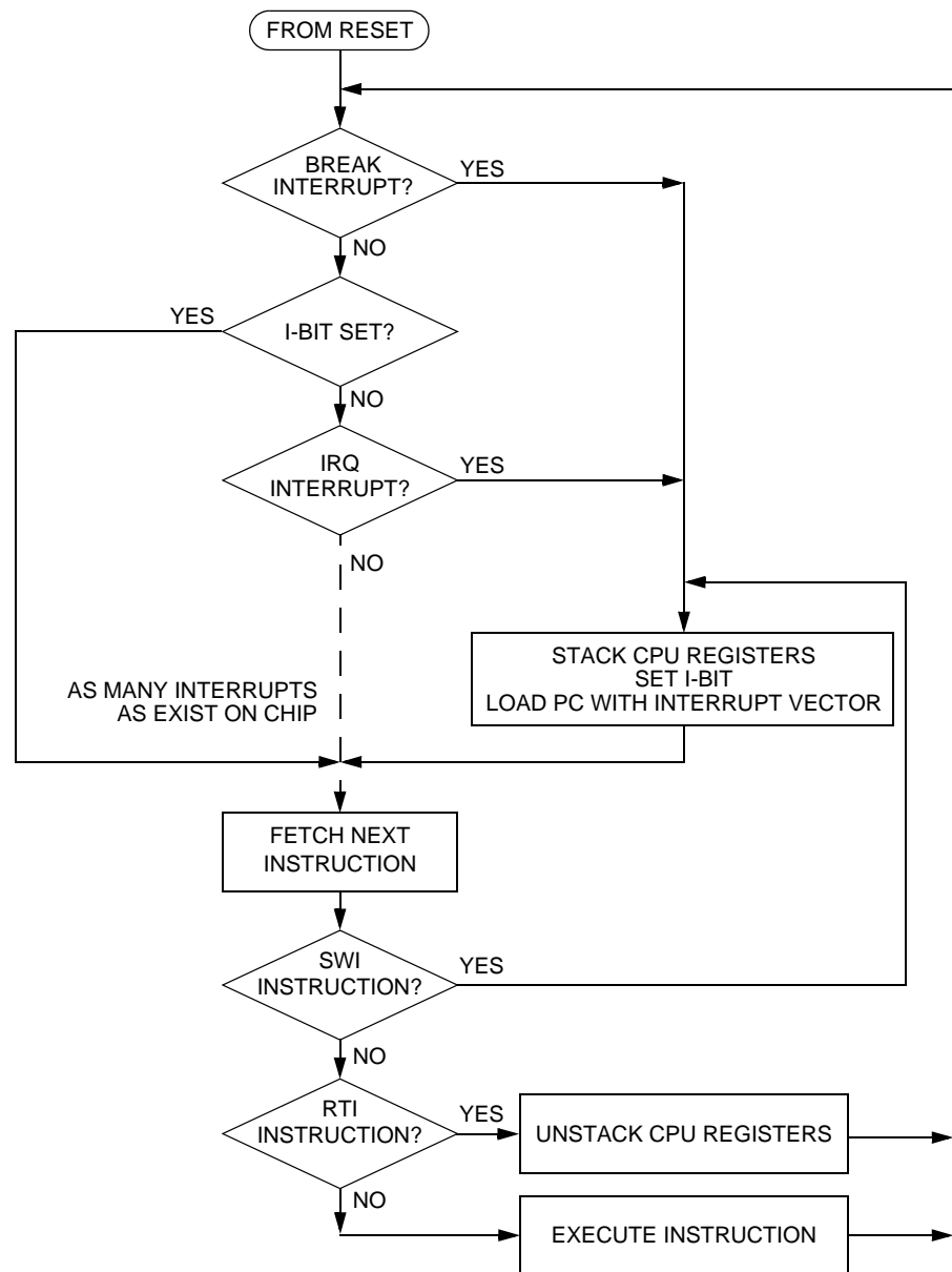
Figure 9-10. Interrupt Processing
