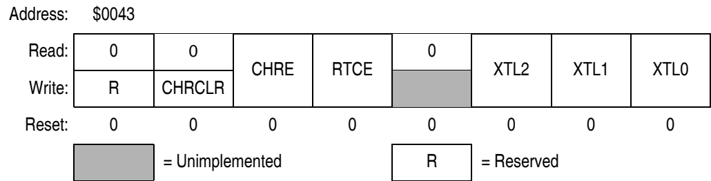
Figure 12-4. RTC Control Register 2 (RTCCR2)
