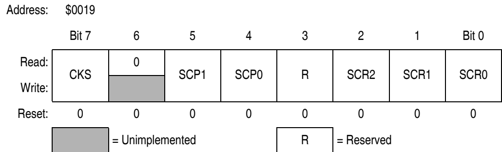
Figure 13-19. SCI Baud Rate Register (SCBR)
