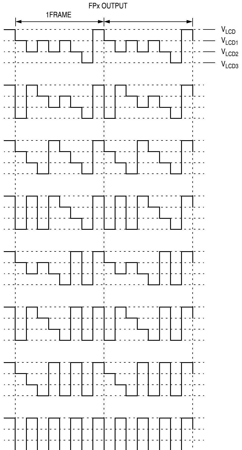
Figure 16-11. 1/4 Duty LCD Frontplane Driver Waveforms (continued)
