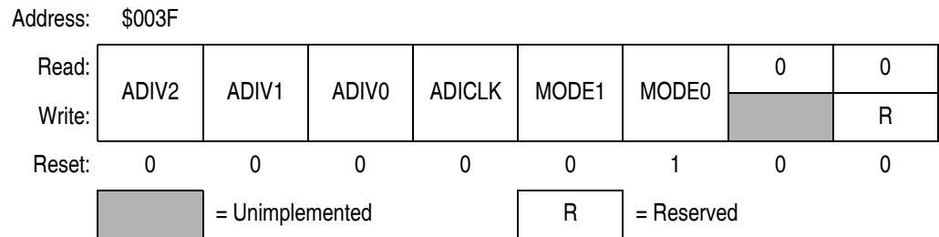
Figure 15-9. ADC Clock Control Register (ADICLK)
